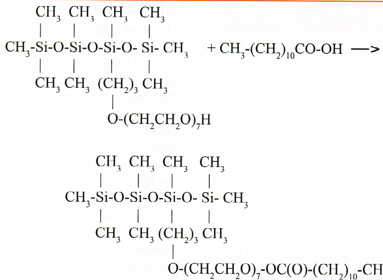
Figure 11. Esterification reaction of dimethicone copolyol with a fatty acid to produce a silicone ester
